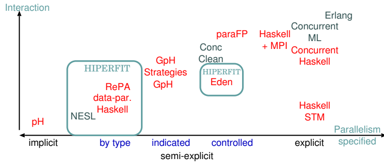
Fig. 2. Parallel Haskell and other functional languages classified
